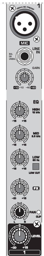
Fig. 2.1: Connectors and controls on the mono channels
