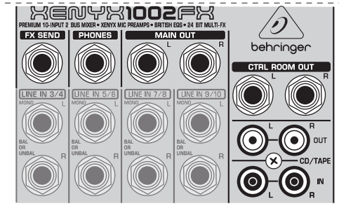
Fig. 2.3: Connectors of the main section
