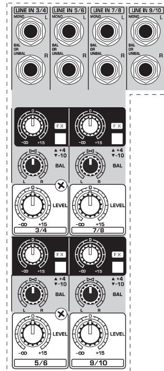
Fig. 2.2: Connectors and controls on the stereo channels
